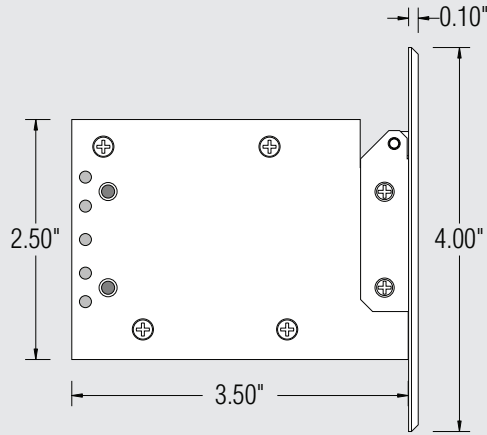
SIDE VIEW (BRACKETS REMOVED)
