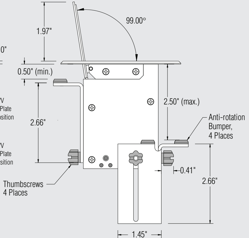
SIDE VIEW WITH BRACKETS
