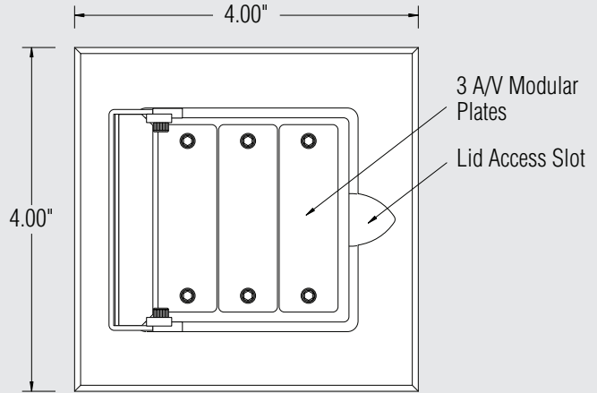
TOP VIEW (LID OPEN)
