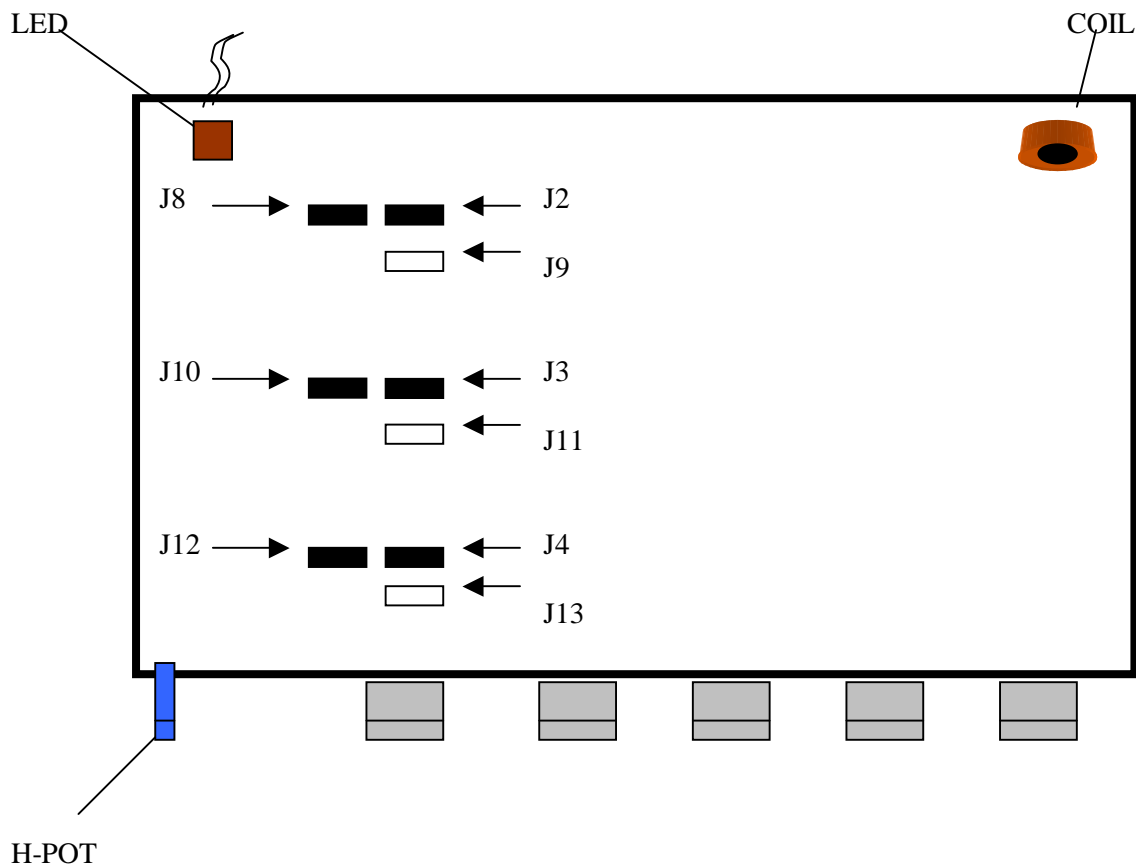
DIAGRAM 1-1 IN3264 BOARD DEFAULT
